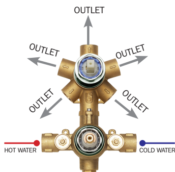
Concealed body for Universal thermostatic mixer 1/2" connections Z00125 with 2-5 ways diverter
