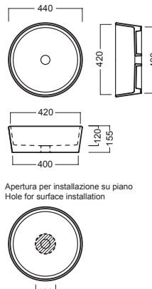
lavabo 07:00 washbasin 07:00
