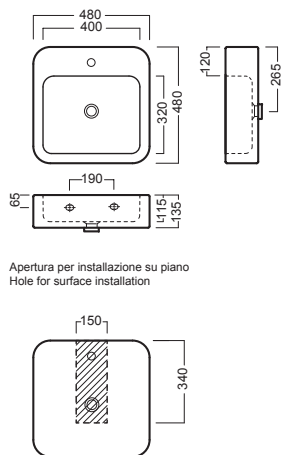
lavabo 09:00 washbasin 09:00
