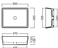
lavabo 11:00 washbasin 11:00
