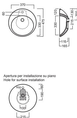
lavabo 02:00 washbasin 02:00
