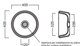
lavabo 40 washbasin 40
