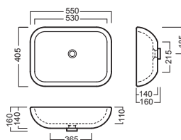
lavabo 17:00 washbasin 17:00
