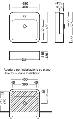
lavabo 09:30 washbasin 09:30
