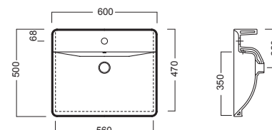
lavabo 60 washbasin 60
