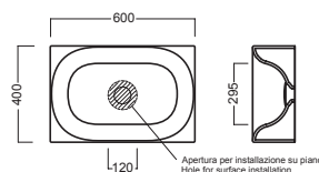
lavabo 60 washbasin 60
