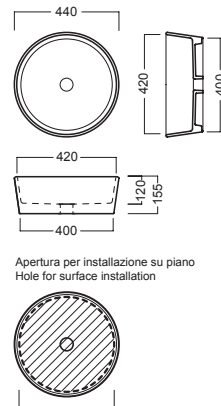
lavabo 07:15 washbasin 07:00
